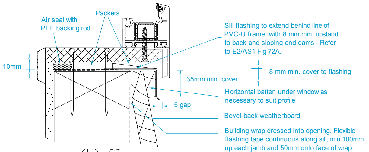
(b) SILL
