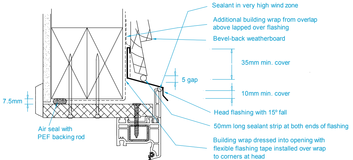
(a) HEAD
