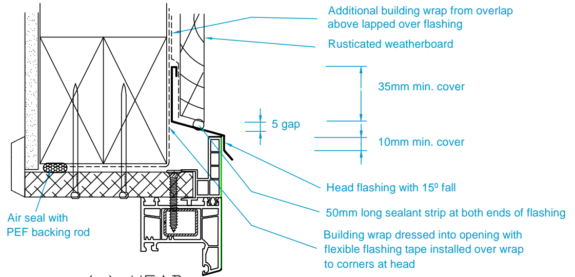
(a) HEAD
