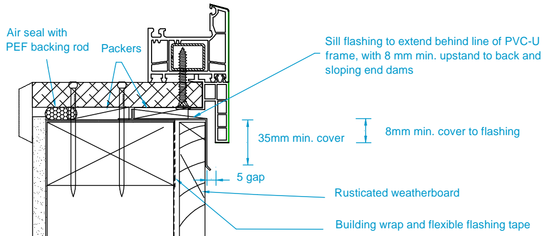
(b) SILL
