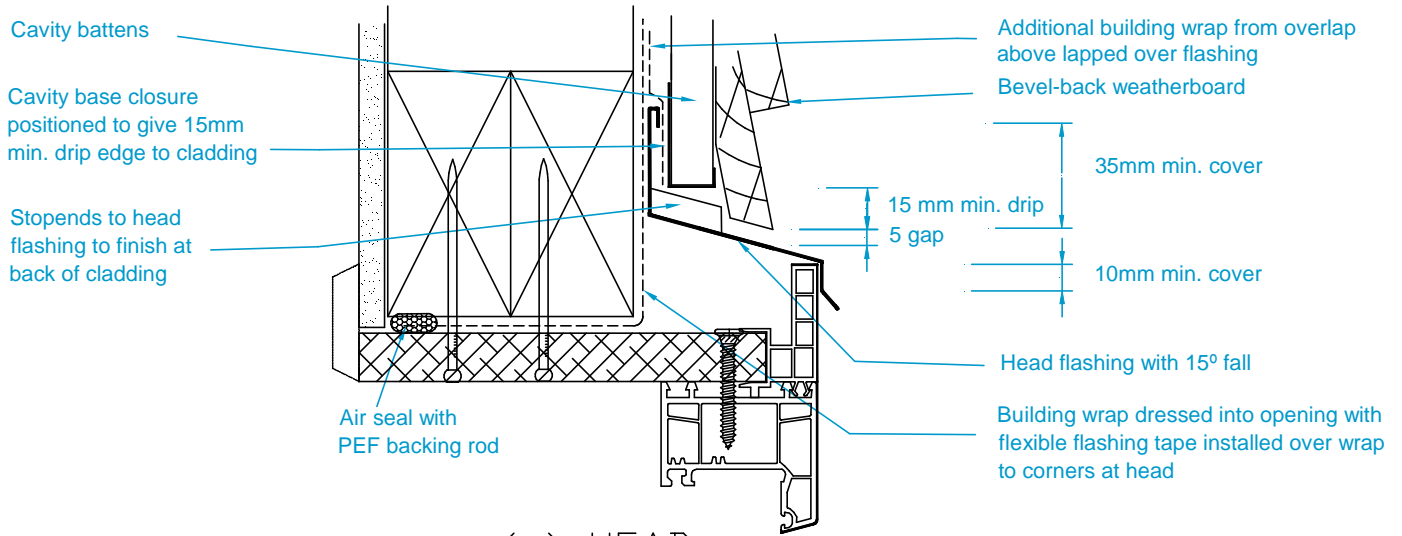
(a) HEAD
