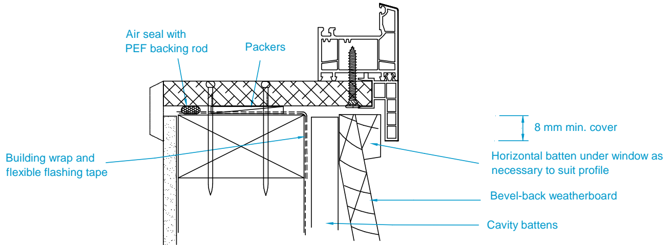
(b) SILL
