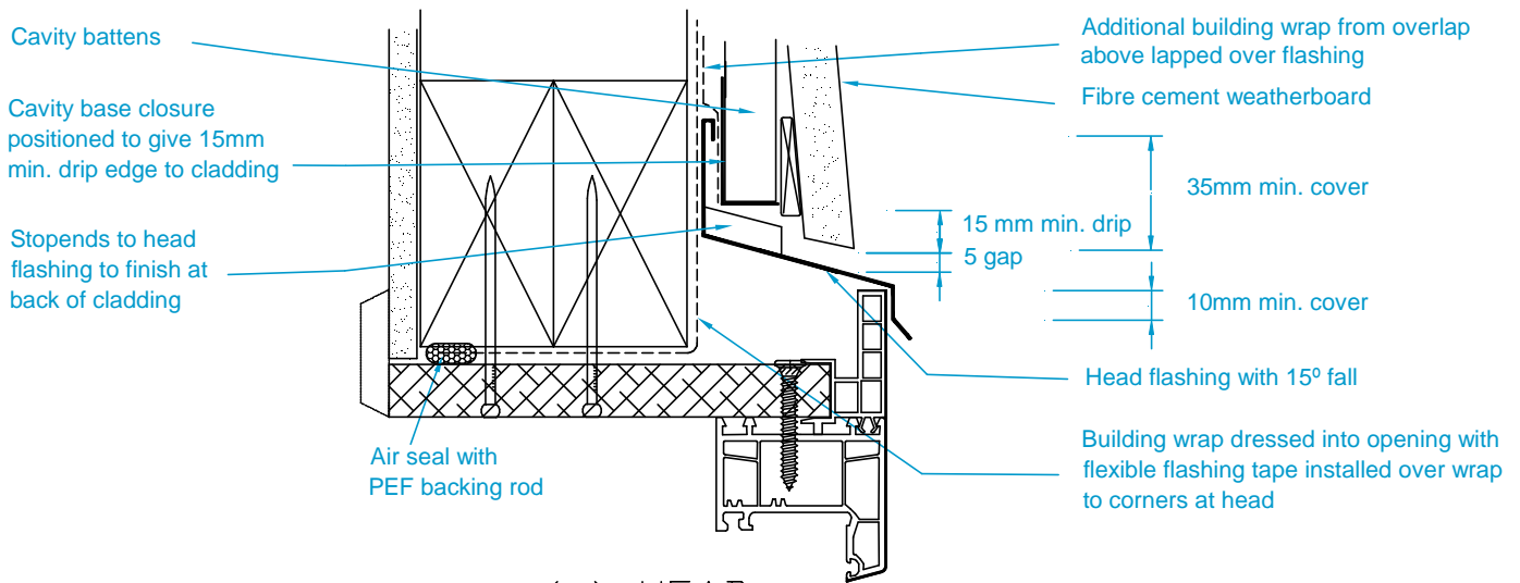
(a) HEAD
