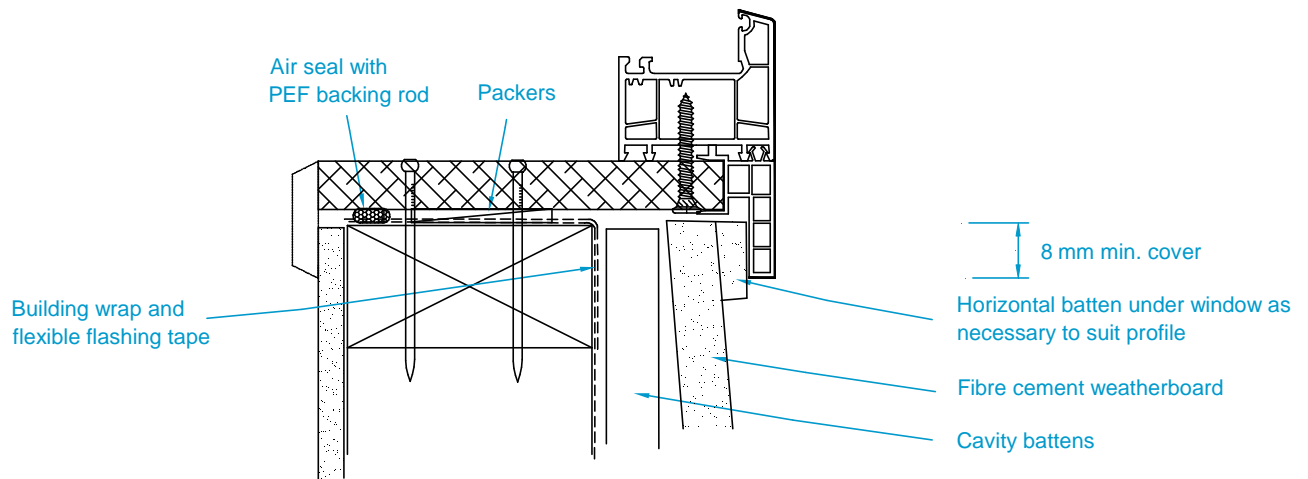
(b) SILL
