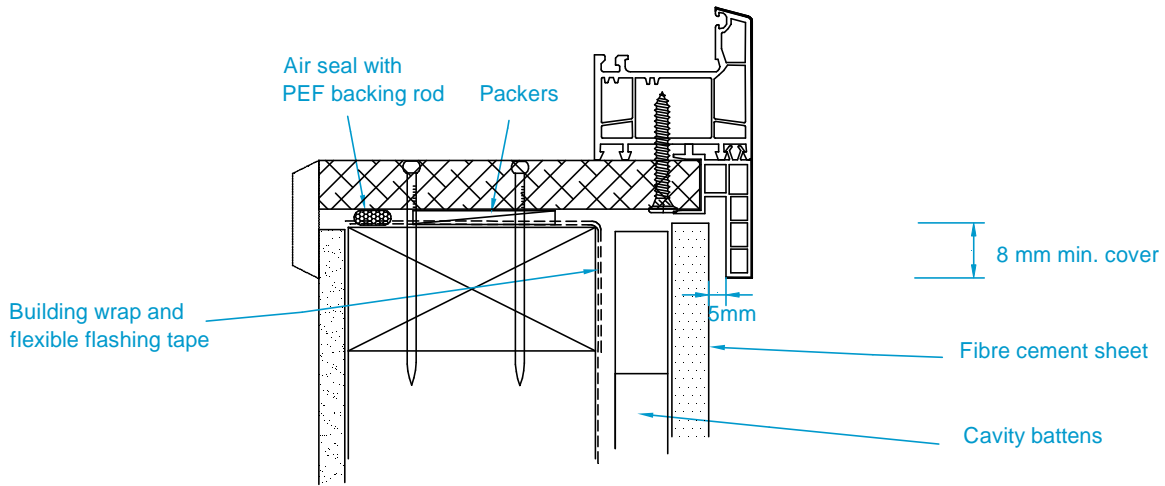
(b) SILL
