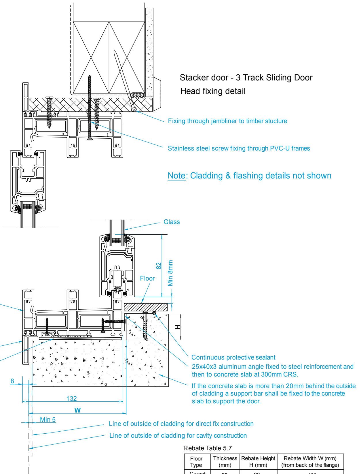
Stacker door - 3 Track Sliding Door Sill rebate detail
